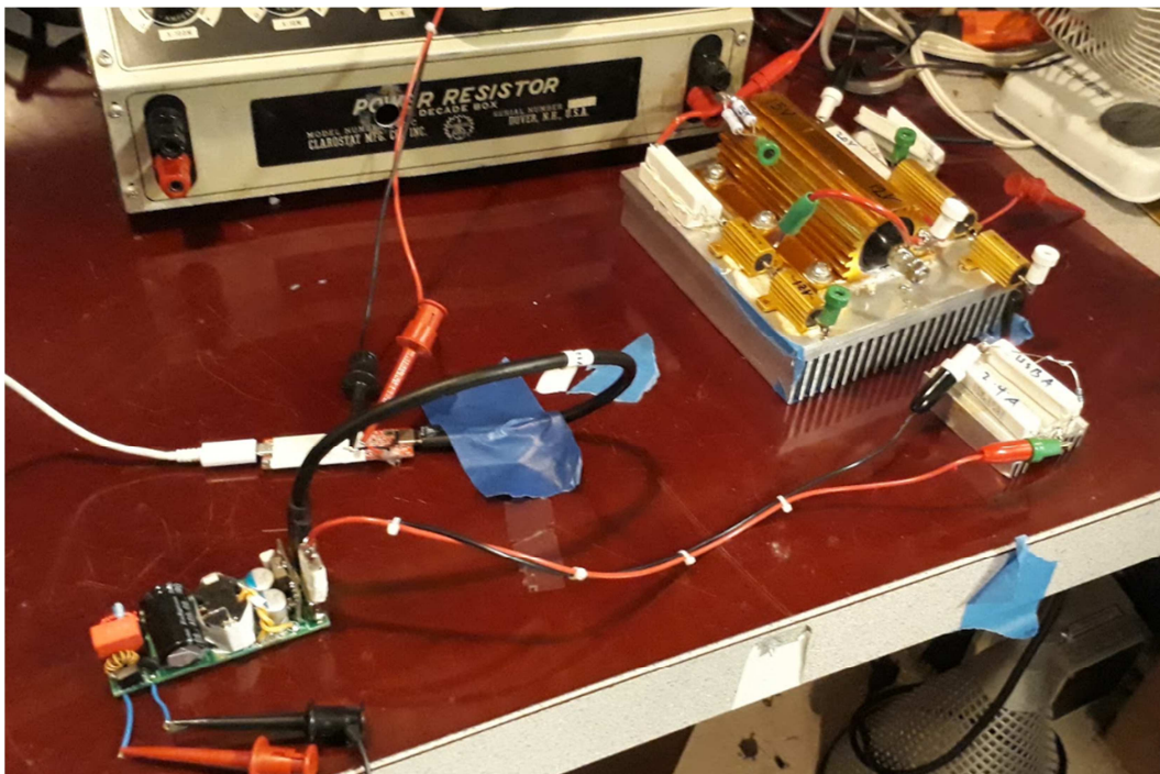
Figure 145 – Conducted EMI Test Set-up.
