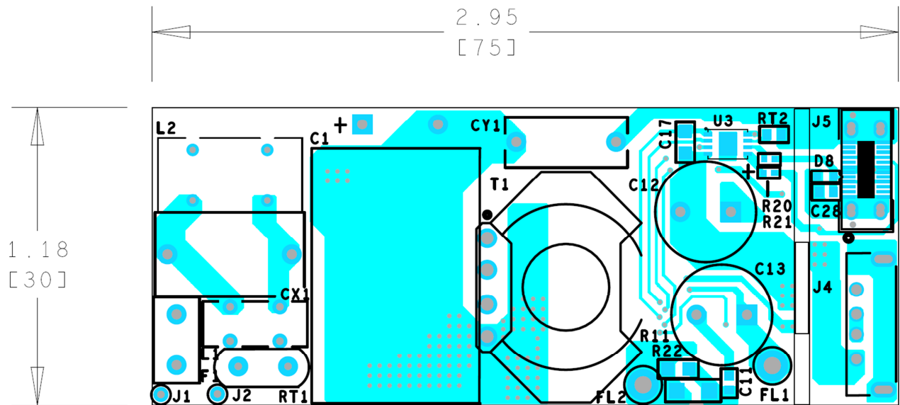
Figure 8 – Top Side.
