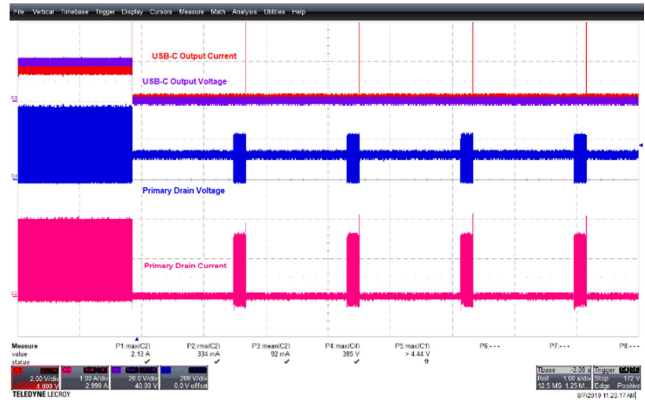
Figure 120 – 265 VAC 50 Hz, USB-C Full Load Short. CH1(Red): I_{USB-C} , 2 A / div., 1 s / div. CH2(Pink): I_{DRAIN} , 1 A / div. CH3(Violet): V_{USB-C} , 20 V / div. CH4(Blue): V_{DRAIN} , 200 V / div.
