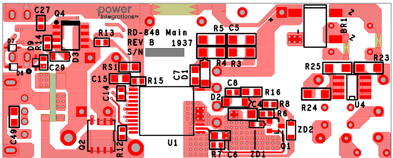
Figure 9 – Bottom Side.
