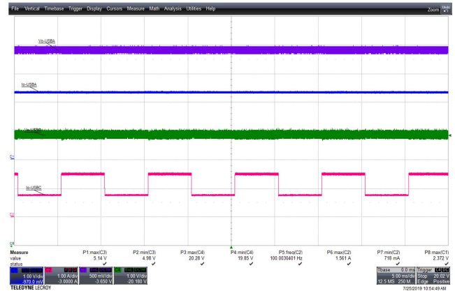
Figure 100 – 265 VAC 50 Hz, 0.75-1.5 A USB-C Transient. CH1(Blue): I_{USB-A} , 1 V / div., 5 ms / div. CH2(Pink): I_{USB-C} , 1 A / div. CH3(Violet): V_{USB-A} , 0.5 V / div. CH4(Green): V_{USB-C} , 1 V / div.
