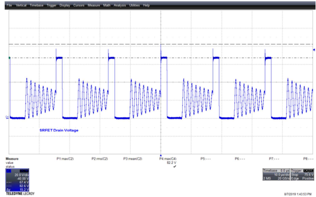
Figure 136 – 265 VAC 50 Hz, V_{USB-C} = 20 V Full Normal. V_{DRAIN} , 20 V / div., 10 \mu s / div. V_{DS} = 82.2 V.
