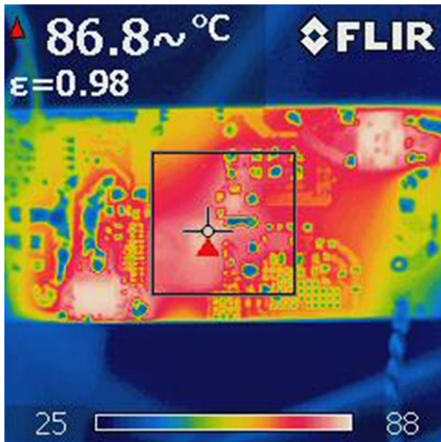
Figure 58 – InnoSwitch3-Pro: 86.8 °C.
