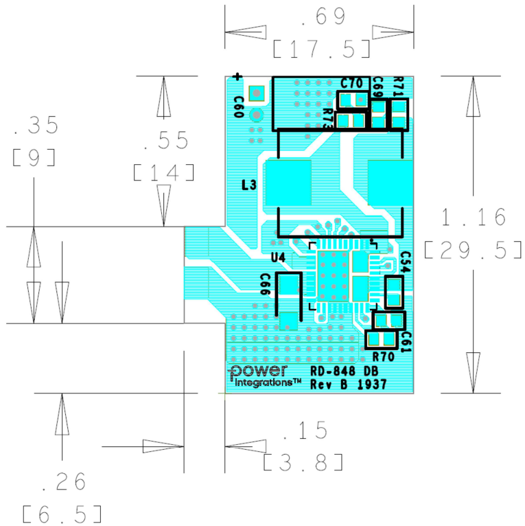
Figure 10 – Top Side.
