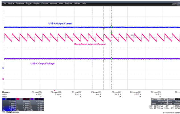
Figure 127 – 90 VAC 60 Hz, USB-A Full Load Short CH1(Blue): I_{USB-Ar} 1 A / div., 10 \mu\text{s} / div. CH2(Pink): I_{L3r} 1 A / div. CH3(Violet): V_{USB-C} , 10 V / div.
