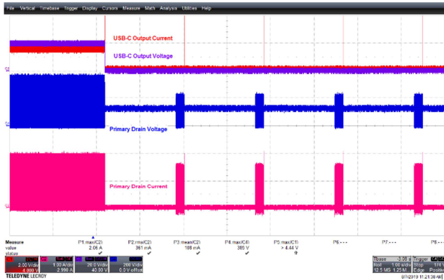
Figure 119 – 90 VAC 60 Hz, USB-C Full Load Short. CH1(Red): I_{USB-C} , 2 A / div., 1 s / div. CH2(Pink): I_{DRAIN} , 1 A / div. CH3(Violet): V_{USB-C} , 20 V / div. CH4(Blue): V_{DRAIN} , 200 V / div.
