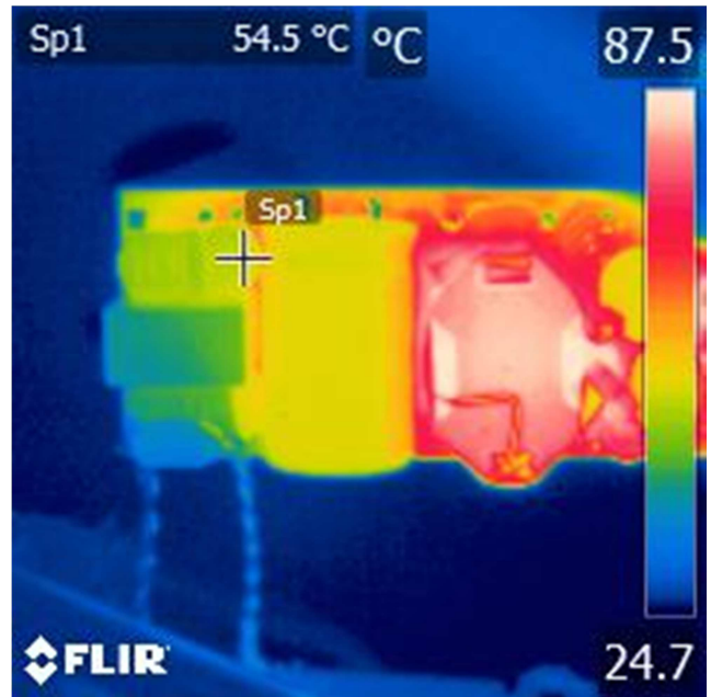
Figure 55 – Input CMC (L2): 54.5 °C.
