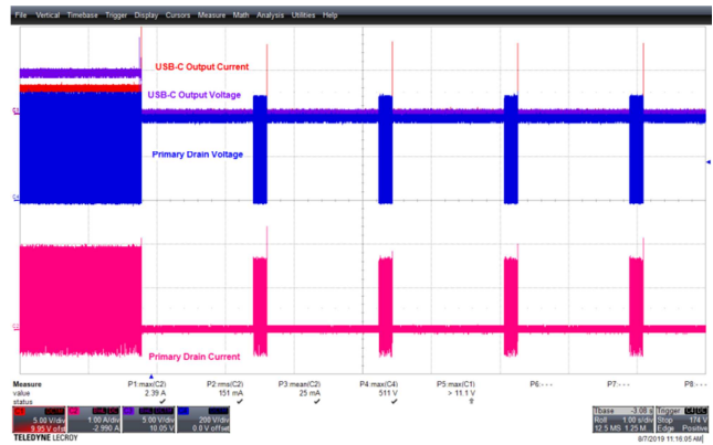
Figure 118 – 265 VAC 50 Hz, USB-C Full Load Short. CH1(Red): I_{USB-C} , 5 A / div., 1 s / div. CH2(Pink): I_{DRAIN} , 1 A / div. CH3(Violet): V_{USB-C} , 5 V / div. CH4(Blue): V_{DRAIN} , 200V / div.
