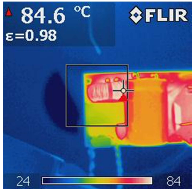
Figure 63 – Input CMC (L2): 84.6 °C.
