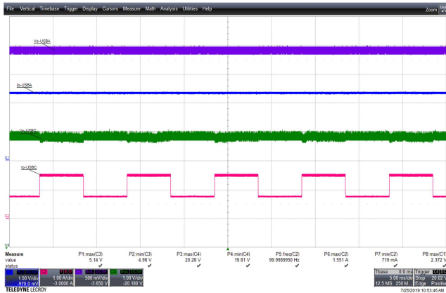
Figure 99 – 90 VAC 60 Hz, 0.75-1.5 A USB-C Transient. CH1(Blue): I_{USB-A} , 1 A / div., 5 ms / div. CH2(Pink): I_{USB-C} , 1 A / div. CH3(Violet): V_{USB-A} , 0.5 V / div. CH4(Green): V_{USB-C} , 1 V / div.
