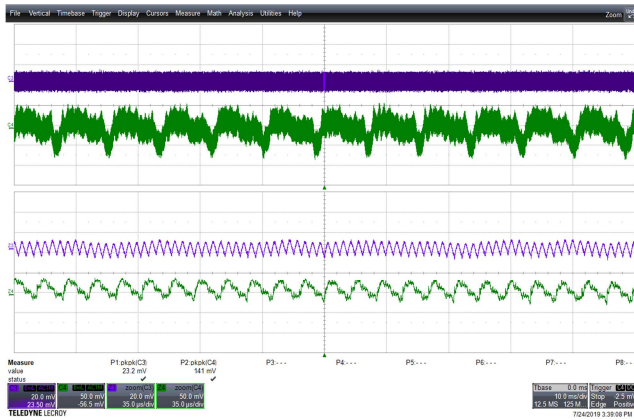
Figure 115 – 90 VAC 60 Hz, Full Load Normal. Upper: V_{USB-A} , 50 mV / div., 10 ms/div. Lower: V_{USB-C} , 50 mV / div. V_{RIPPLE(USB-A)} = 23.2\text{ mVpp} . V_{RIPPLE(USB-C)} = 141\text{ mVpp} .
