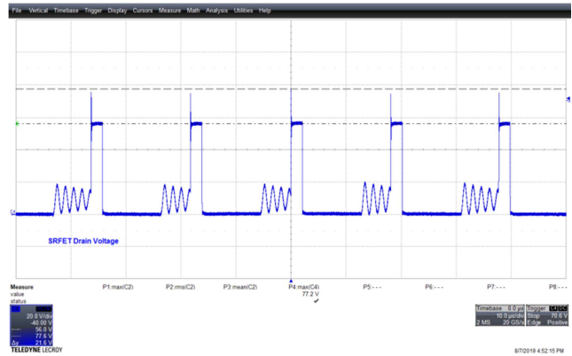
Figure 142 – 265 VAC 50 Hz, V_{USB-C} = 9 V Full Normal. V_{DRAIN} , 20 V / div., 10 \mu s / div. V_{DS} = 77.2 V.
