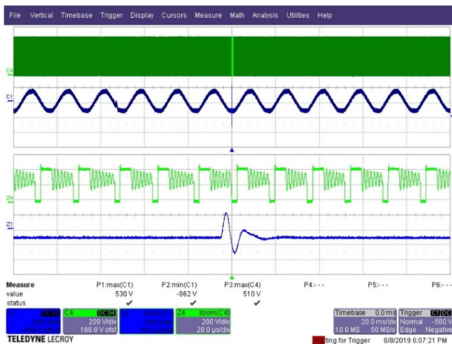
Figure 164 – 230 VAC 50 Hz, 2.5kV Ring Wave L/N. Injection Phase: 90°. Upper: V DRAIN , 200 V / div. Lower: V IN , 500 V / div., 20 ms / div. VDS = 510 V.
