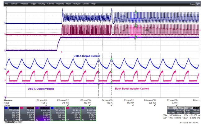
Figure 124 – 265 VAC 60 Hz, USB-A Start-up Short. CH1(Blue): I_{USB-Ar} , 0.5 A / div., 5 ms / div. CH2(Pink): I_{L3r} , 1 A / div. CH3(Violet): V_{USB-C} , 2 V / div.
