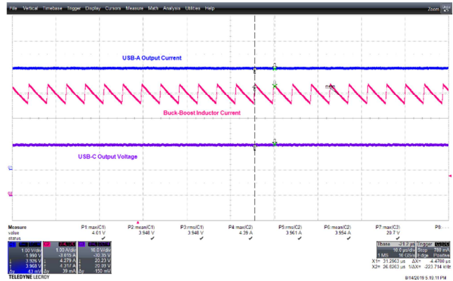
Figure 128 – 265 VAC 60 Hz, USB-A Full Load Short. CH1(Blue): I_{USB-Ar} 1 A / div., 10 \mu\text{s} / div. CH2(Pink): I_{L3r} 1 A / div. CH3(Violet): V_{USB-C} , 10 V / div.
