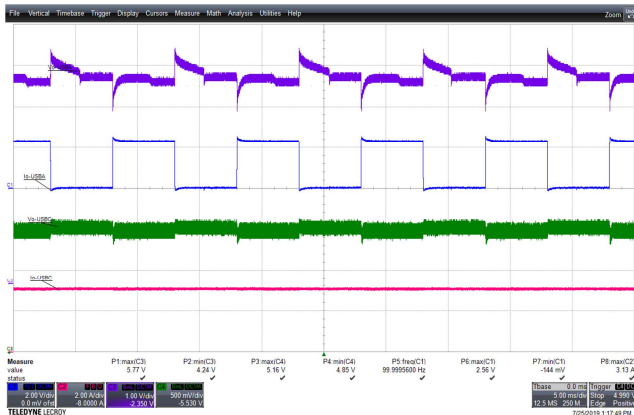
Figure 101 – 90 VAC 60 Hz, 0-2.4 A USB-A Transient. CH1(Blue): I_{USB-A} , 2 A / div., 5 ms / div. CH2(Pink): I_{USB-C} , 2 A / div. CH3(Violet): V_{USB-A} , 1 V / div. CH4(Green): V_{USB-C} , 0.5 V / div.
