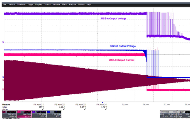
Figure 166 – Brown-Out from 230 V to 0 V. Slew Rate: 0.5 V / s. CH1(Brown): V_{IN} , 200 V / div. CH2(Pink): I_{USB-C} , 1 A / div., 50 s / div. CH3(Violet): V_{USB-A} , 2 V / div. CH4(Blue): V_{USB-C} , 2 V / div.
