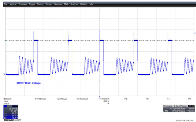
Figure 138 – 265 VAC 50 Hz, V_{USB-C} = 15 V Full Normal. V_{DRAIN} , 20 V / div., 10 \mu s / div. V_{DS} = 80.6 V.
