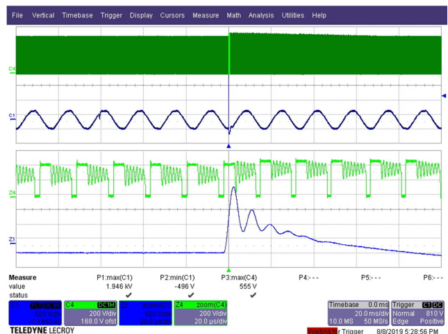
Figure 163 – 230 VAC 50 Hz, 2 kV Differential Surge L/N. Injection Phase: 270° Upper: V DRAIN , 200 V / div. Lower: V IN , 500 V / div., 20 ms / div. V DS = 555 V.
