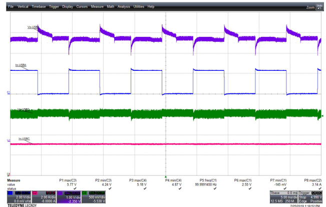
Figure 102 – 265 VAC 50 Hz, 0-2.4 A USB-A Transient. CH1(Blue): I_{USB-A} , 2 V / div., 5 ms / div. CH2(Pink): I_{USB-C} , 2 A / div. CH3(Violet): V_{USB-A} , 1 V / div. CH4(Green): V_{USB-C} , 0.5 V / div.
