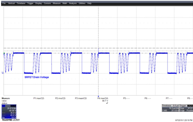
Figure 135 – 90 VAC 60 Hz, V_{USB-C} = 20 V Full Normal. V_{DRAIN} , 20 V / div., 10 \mu s / div. V_{DS} = 45 V.
