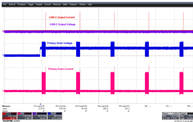
Figure 121 – 90 VAC 60 Hz, USB-C Full Load Short. CH1(Red): I_{USB-C} , 5 A / div., 1 s / div. CH2(Pink): I_{DRAIN} , 1 A / div. CH3(Violet): V_{USB-C} , 20 V / div. CH4(Blue): V_{DRAIN} , 200 V / div.
