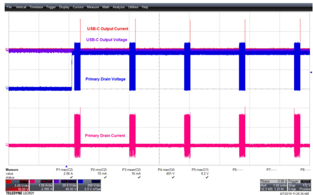
Figure 122 – 265 VAC 50 Hz, USB-C Full Load Short. CH1(Red): I_{USB-C} , 5 A / div., 1 s / div. CH2(Pink): I_{DRAIN} , 1 A / div. CH3(Violet): V_{USB-C} , 20 V / div. CH4(Blue): V_{DRAIN} , 200 V / div.
