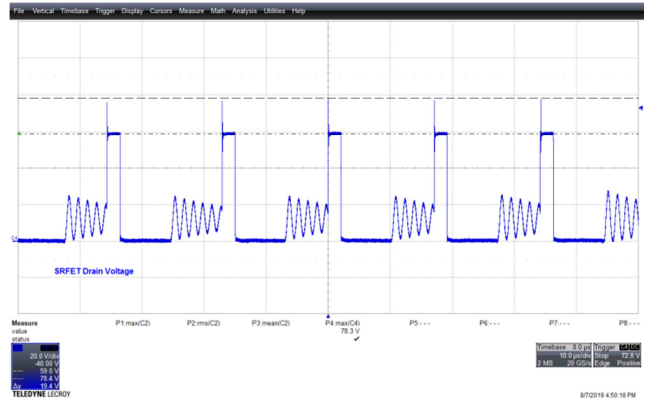
Figure 140 – 265 VAC 50 Hz, V_{USB-C} = 12 V Full Normal. V_{DRAIN} , 20 V / div., 10 \mu s / div. V_{DS} = 78.3 V.
