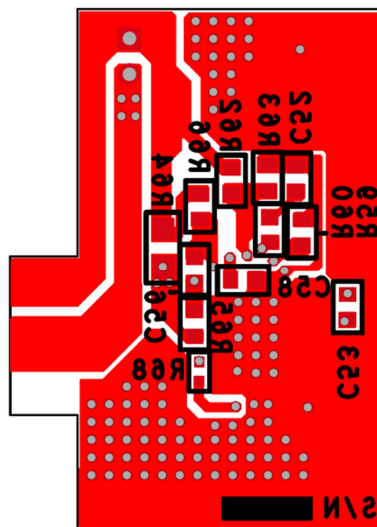
Figure 11 – Bottom Side.
