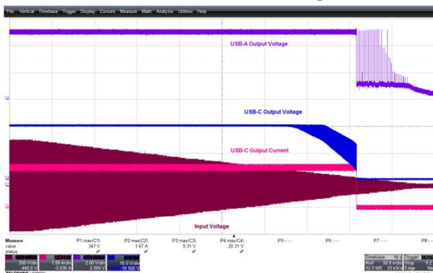
Figure 168 – Brown-Out from 230 V to 0 V. Slew Rate: 0.5 V / s. CH1(Brown): V_{IN} , 200 V / div. CH2(Pink): I_{USB-C} , 1 A / div., 50 s / div. CH3(Violet): V_{USB-A} , 2 V / div. CH4(Blue): V_{USB-C} , 10 V / div.
