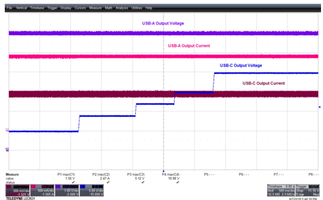
Figure 86 – 265 VAC 60 Hz, 5 V - 9 V - 12 V - 15 V - 20 V Step. CH1(Brown): I_{USB-C} , 500 mA / div., CH2(Pink): I_{USB-A} , 500 mA / div. CH3(Violet): V_{USB-A} , 1 V / div. 500 ms / div. CH4(Blue): V_{USB-C} , 5 V / div. Remark: No overshoot/undershoot.
