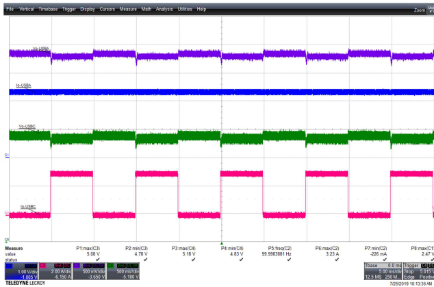
Figure 93 – 90 VAC 60 Hz, 0-3 A USB-C Transient Load CH1(Blue): I_{USB-A} , 1 A / div., 5 ms / div. CH2(Pink): I_{USB-C} , 2 A / div. CH3(Violet): V_{USB-A} , 0.5 V / div. CH4(Green): V_{USB-C} , 0.5 V / div.
