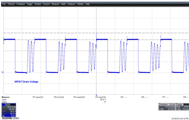
Figure 137 – 90 VAC 60 Hz, V_{USB-C} = 15 V Full Normal. V_{DRAIN} , 20 V / div., 10 \mu s / div. V_{DS} = 36.4 V.
