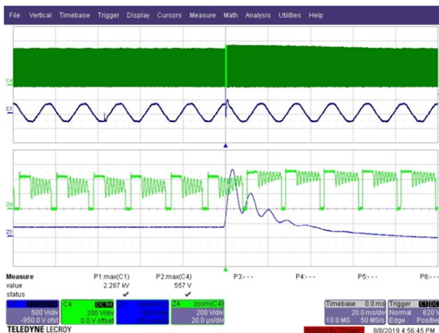
Figure 162 – 230 VAC 50 Hz, 2 kV Differential Surge L/N. Injection Phase: 90° Upper: V DRAIN , 200 V / div. Lower: V IN , 500 V / div., 20 ms / div. V DS = 557 V.
