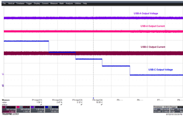
Figure 87 – 90 VAC 60 Hz, 20 V - 15 V - 12 V - 9 V - 5 V. CH1(Brown): I_{USB-C} , 500 mA / div. CH2(Pink): I_{USB-A} , 500 mA / div. CH3(Violet): V_{USB-A} , 1 V / div., 500 ms. CH4(Blue): V_{USB-C} , 5 V / div. Remark: No overshoot/undershoot.
